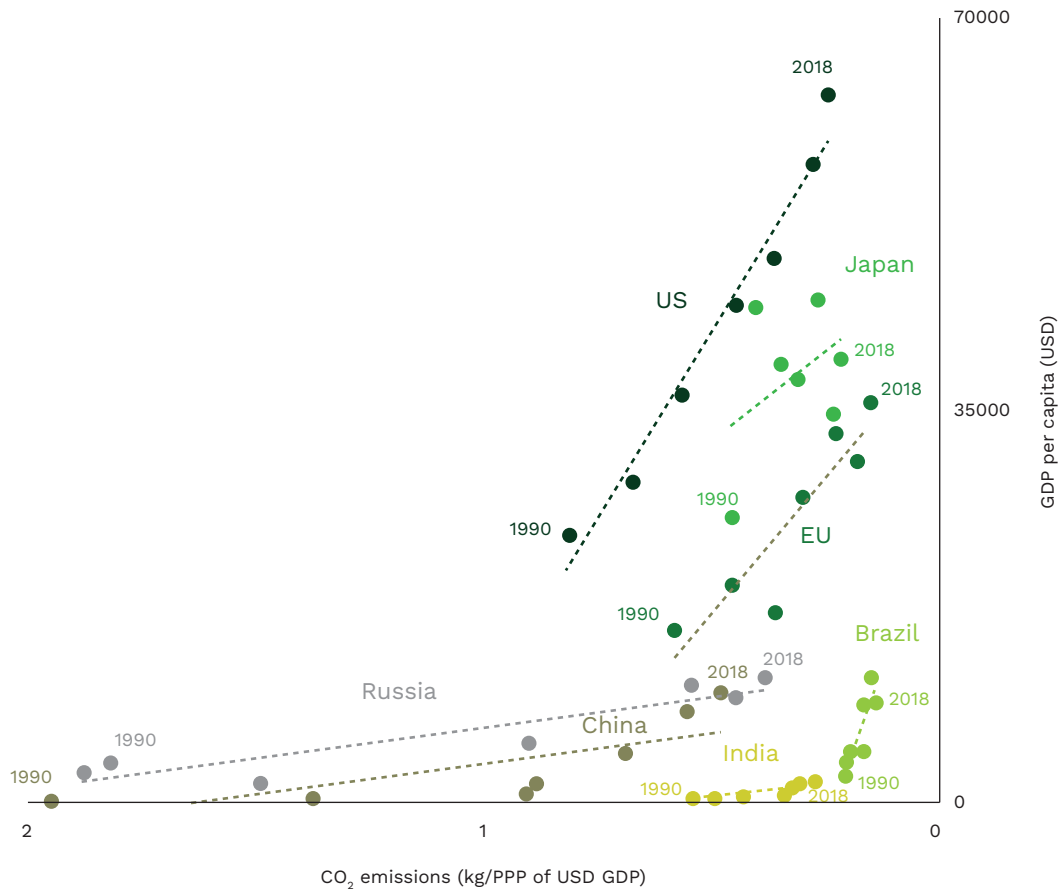
Figure 7. The US and China produce more CO 2 per GDP than the EU CO 2 emissions (in kg/PPP of USD GDP) per GDP per capita in 1990-2018 (in USD)
