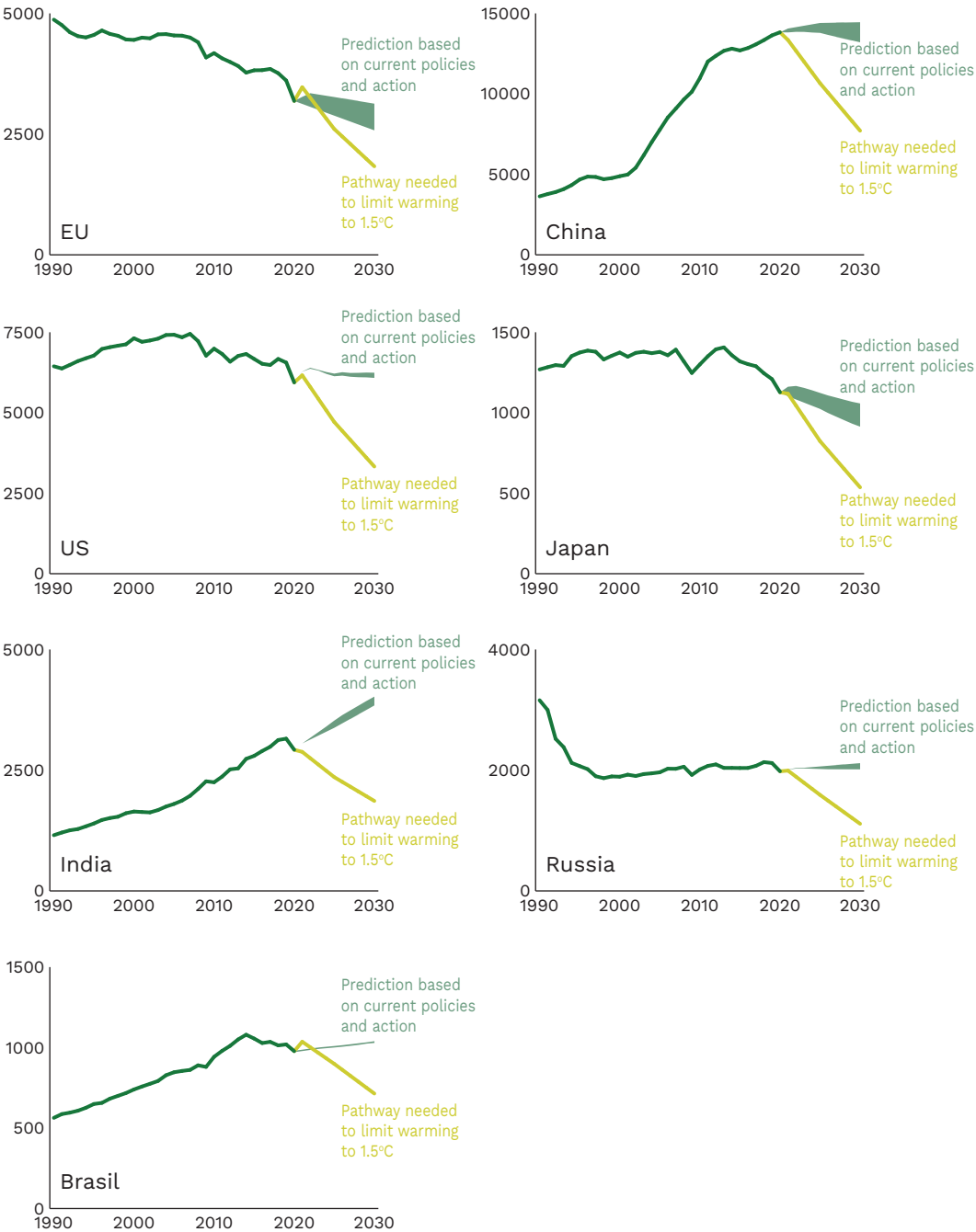
Figure 10. The EU is the closest to the 1.5°C pathway Historical and predicted CO 2 emissions pathways (in MtCO 2 e)
